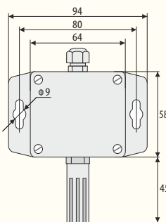
Probe integrated with the enclosure AR250
