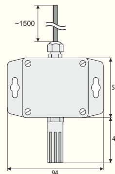
External probe in an enclosure with a wire AR250/3
